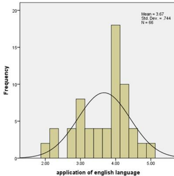
Histogram diagram of Kolmogorov-Smirnov Test
